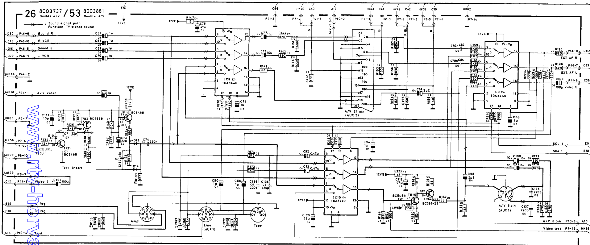
DIAGRAM G DOUBLE A/V CONNECTIONS
